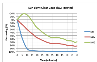
Figure 6 - Pollutant abatement over time in the presence of photocatalysis conditions
