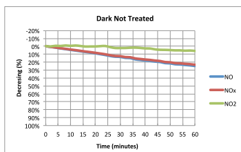
Figure 5 - Pollutant abatement over time in the absence of photocatalysis conditions
